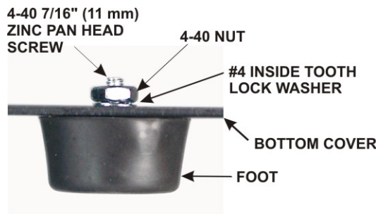
Figure 84. Installing Rear Feet.
