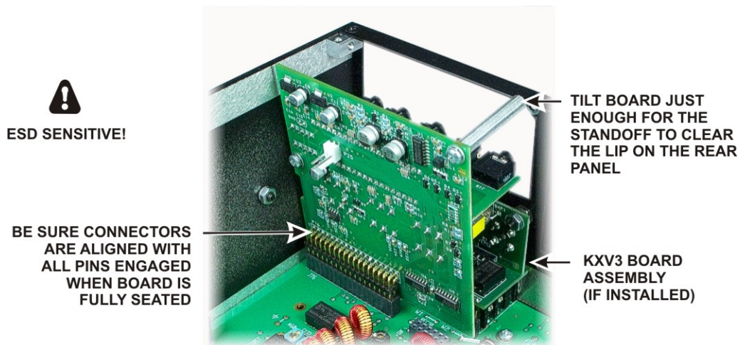
Figure 33. Installing KIO3 Main Board.
