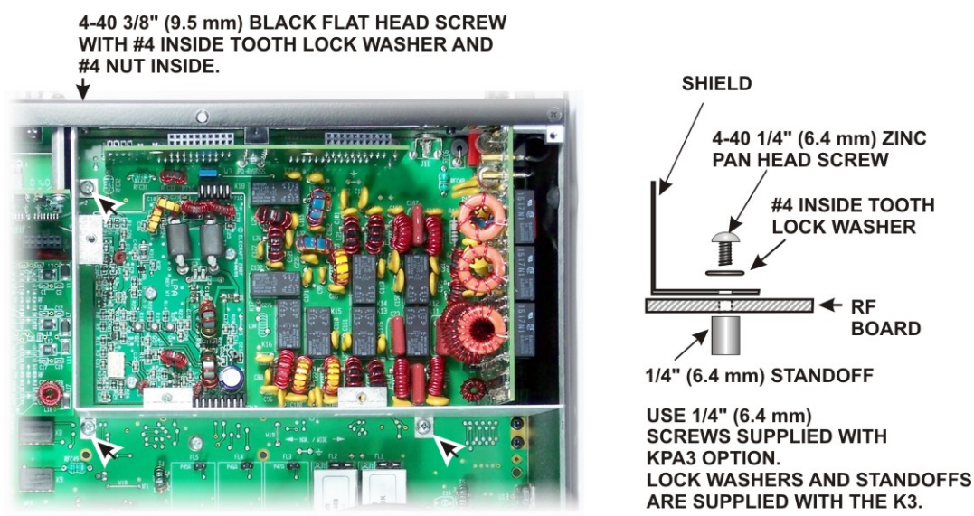
Figure 80. Attaching the KPA3 Shield.
