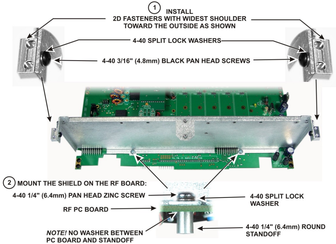
Figure 13. Installing Front Panel Shield.
