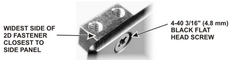
Figure 17. Installing Left Side Panel 2D Fastener.
