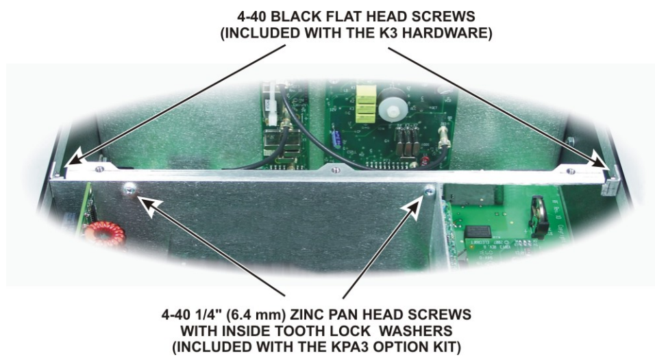
Figure 81. Installing the Chassis Stiffener Bar.
