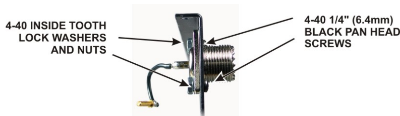
Figure 18. Mounting the ANT1 Connector.
